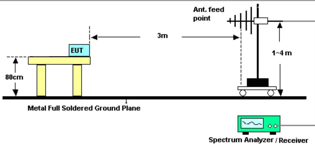
Figure 1. Below 1GHz
