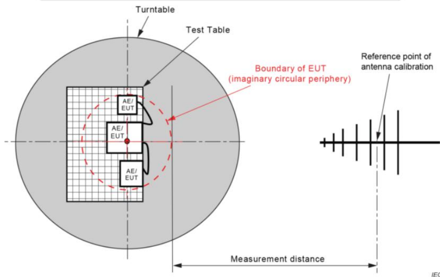
Figure 2. Above 1GHz
