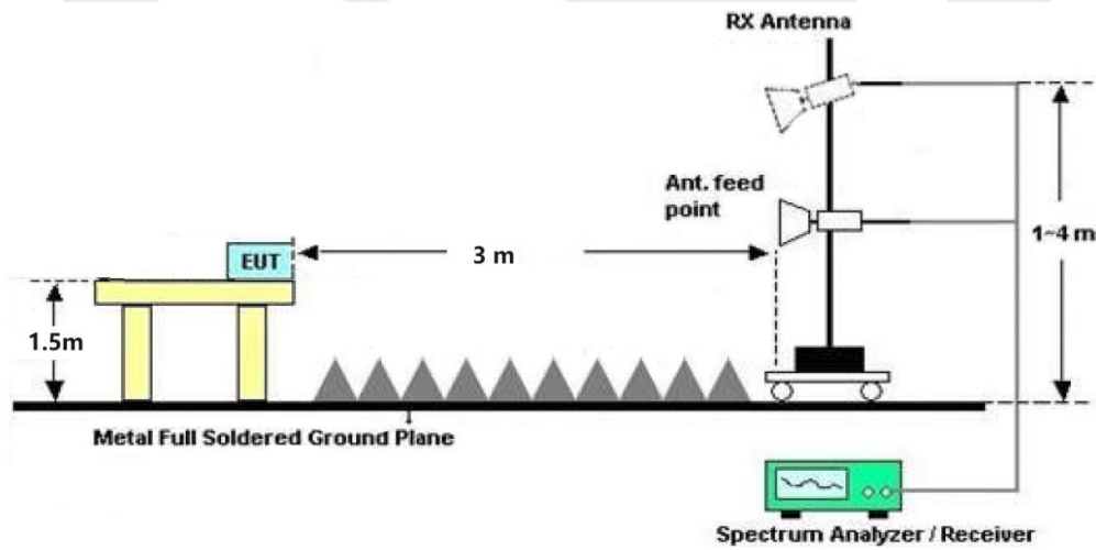
Figure 2. Above 1GHz
