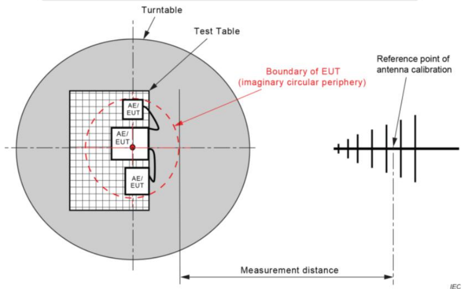
Figure 2. Above 1GHz
