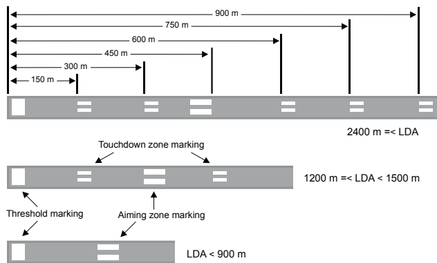
Figure 5.4—Aiming Point and TDZ Marking Examples
