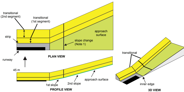
Figure 4.1—Example of OLSs
