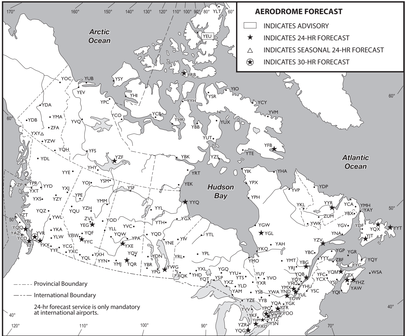
Figure 7.1—TAF Locations
