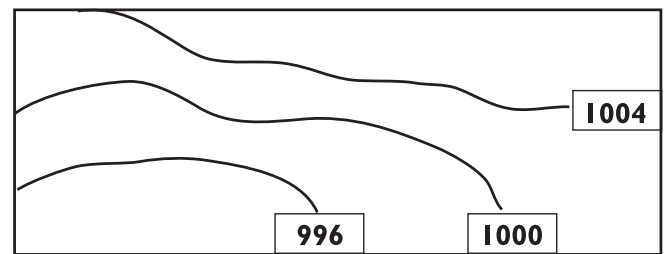
Figure 4.4(g)—Isobars
