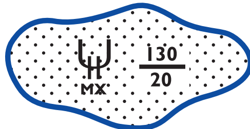
Figure 4.5(b)—Icing
