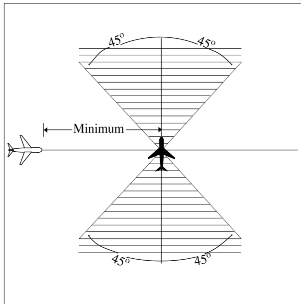
FIG 8-3-2 Crossing Courses
