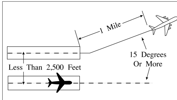
FIG 5-8-2 Simultaneous Departures
