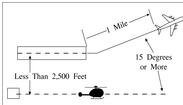
FIG 5-8-3 Simultaneous Departures
