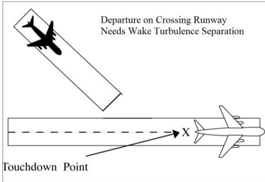
FIG 3-9-20 Converging Runway Separation
