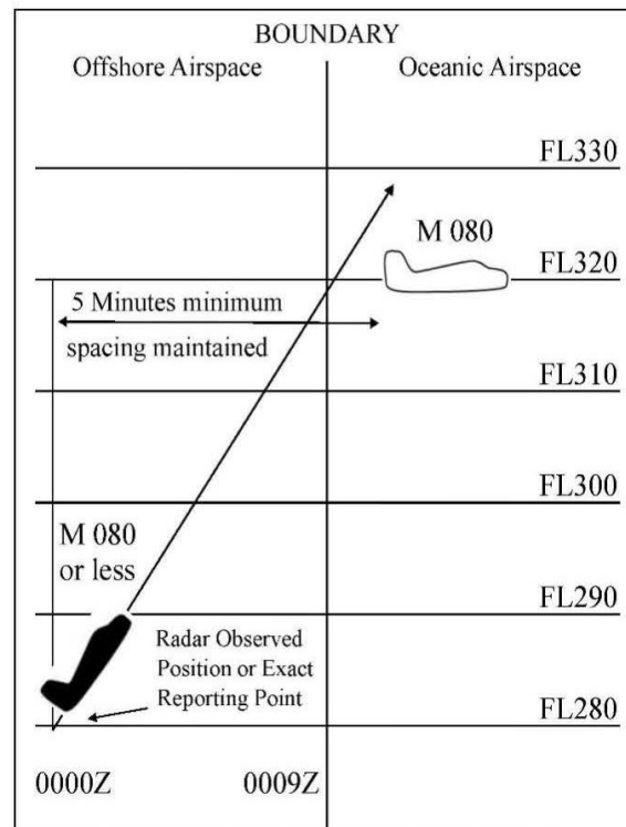
FIG 8-5-3 Transitioning From Offshore to Oceanic Airspace Same Direction
