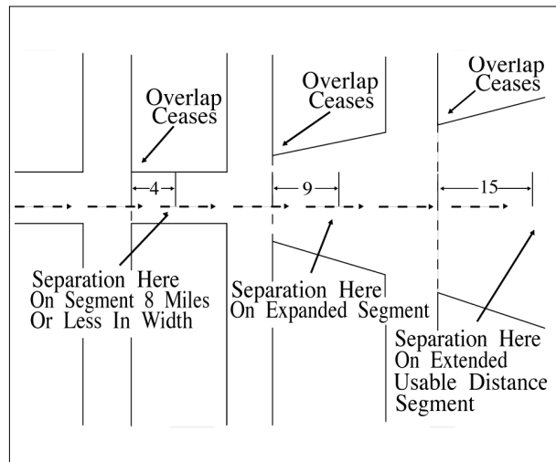
FIG 6–5–8 RNAV Minima
